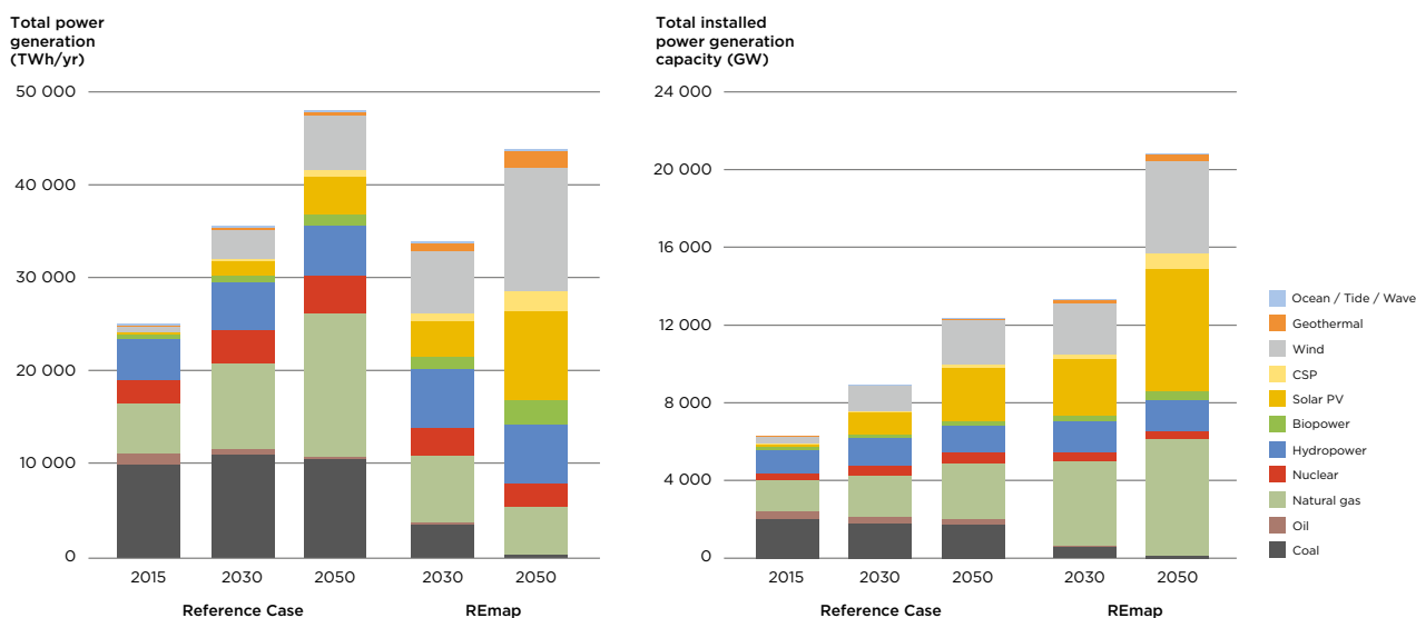
Figure 1: Electricity sector capacity and total electricity generation by technology in the REmap Reference and Doubling cases, 2015-2050
