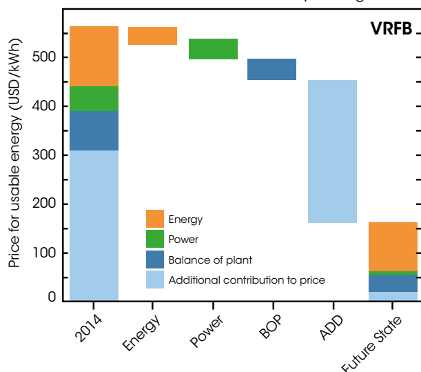
Figure 43: Potential pathway to reach cost-effective vanadium redox flow battery storage
