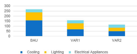
Breakdown of electricity consumption in hot & dry climate (kWh/m 2 /year)
