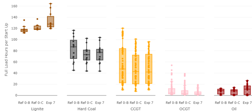
Figure 6.9: Average electricity generated per nameplate capacity between each start up for different conventional technologies in the selected scenarios.
