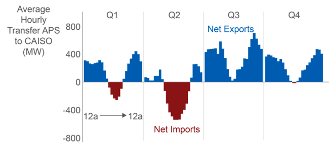
Fig. 8. Average hourly transfer from APS to CAISO in the EIM by quarter in 2018. Figure adapted by Hildebrandt et al. (2019).
