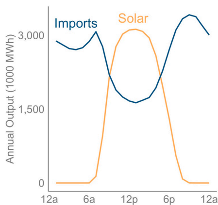
Fig. 6. Daily generation profiles in CAISO for PV and other generation resources.
