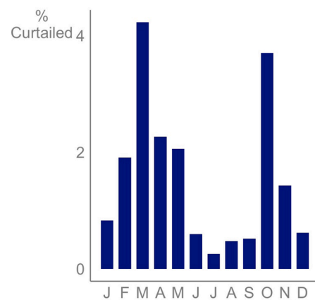
Fig. 4. Percentage of potential PV output curtailed by month in California in 2018.
