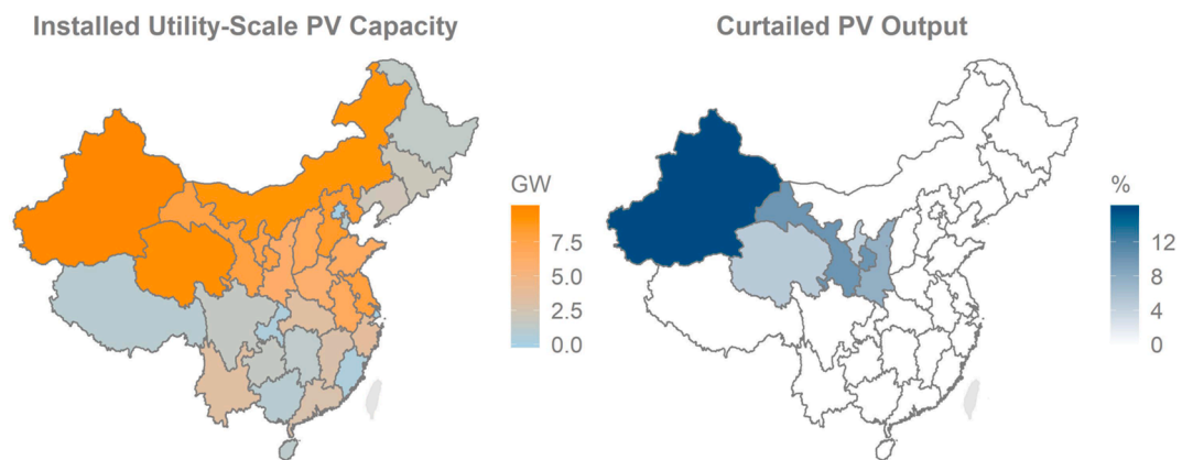
Fig. 3. Province-level installed PV capacity (left) and curtailment (right) in China, based on 2018 data.
