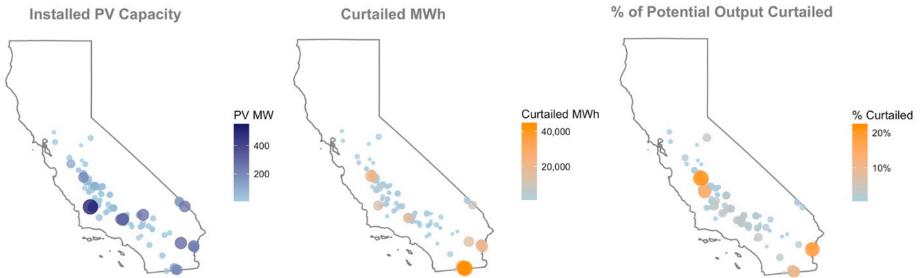
Fig. 5. PV capacity (left), curtailed MWh (center), and estimated curtailment as a percentage of potential output (right), by node in California in 2018. Nodal-level PV capacity and curtailed MWh are based on data provided by CAISO. Curtailment as a percentage of potential output is calculated using assumed PV generation levels based on nodal-level insolation profiles from the National Renewable Energy Laboratory (NREL) National Solar Radiation Data Base.
