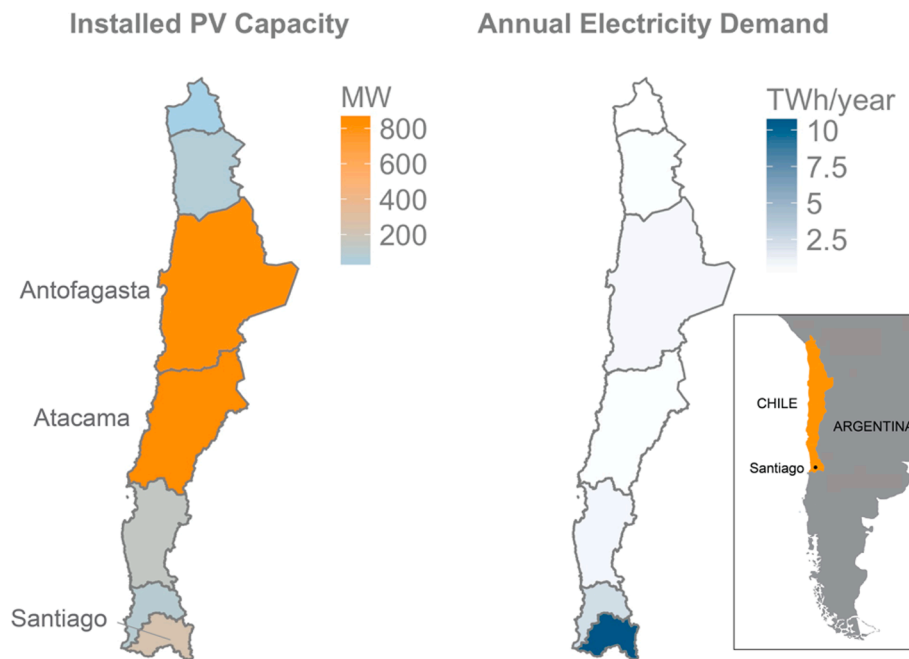
Fig. 2. Region-level installed PV capacity (left) and electricity demand (right) in Chile. Figure based on data from Energía Abierta (2019).
