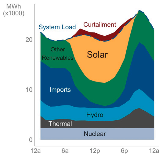
Fig. 1. PV curtailment event on May 13, 2018, in California. Based on data from CAISO (2019a).
