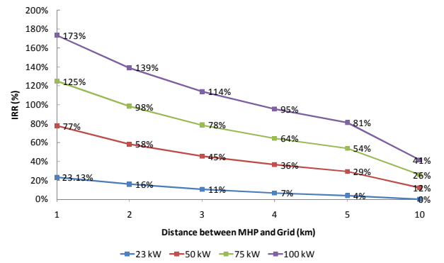
Fig. 9 (a). Internal Rate of Return (IRR) vs Interconnection Distance
