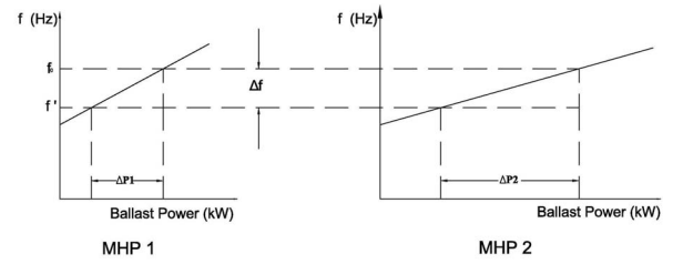
Fig. 5. p-f droop for parallel operation of MHP
