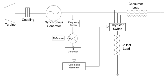
Fig. 3. Control Strategy of ELC practiced in Nepal
