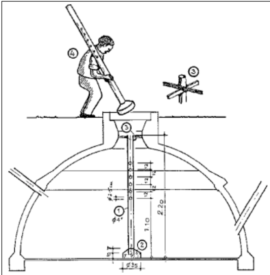
Fig.42: Stand-pipe for gas release
