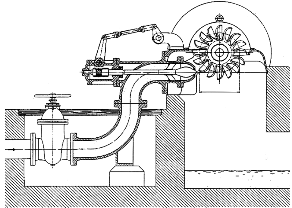
Cross-section of Pelton turbine
