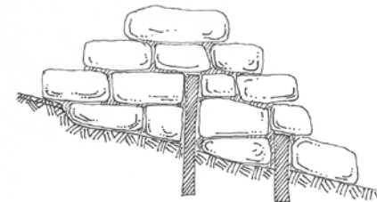
Secure with iron rod against sliding
