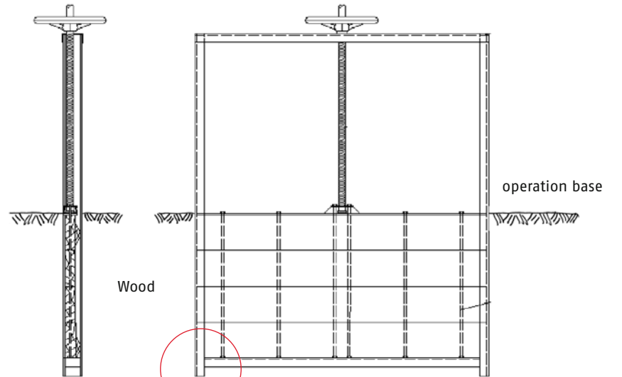
Sliding gate fitted with spindle
