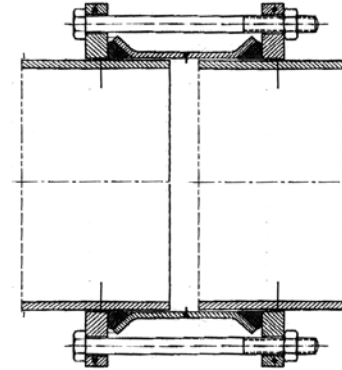
Type dresser: expensive
