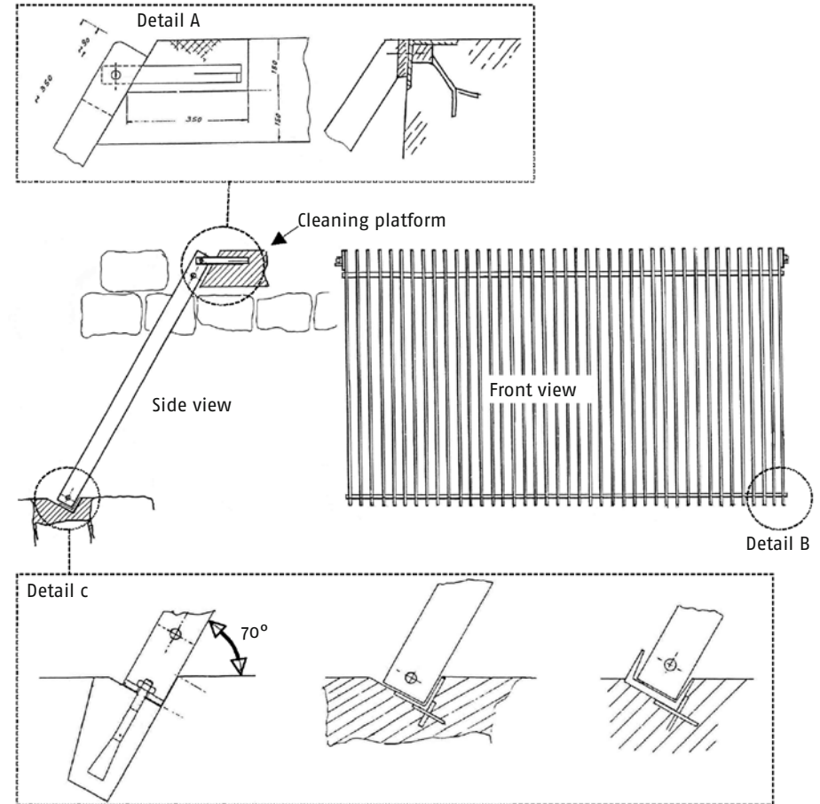
Typical fine trash rack construction
