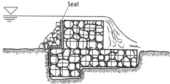
Gabion weir
