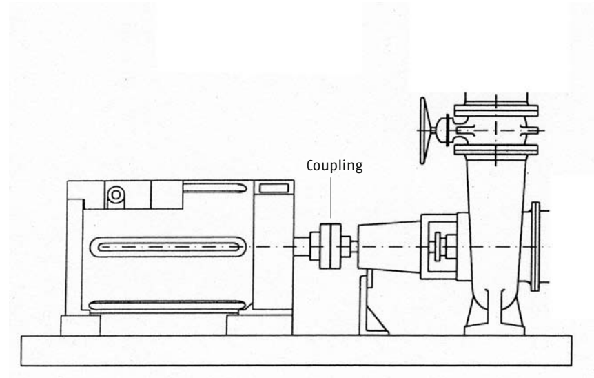
Synchronous generator with pump as turbine (PAT)
