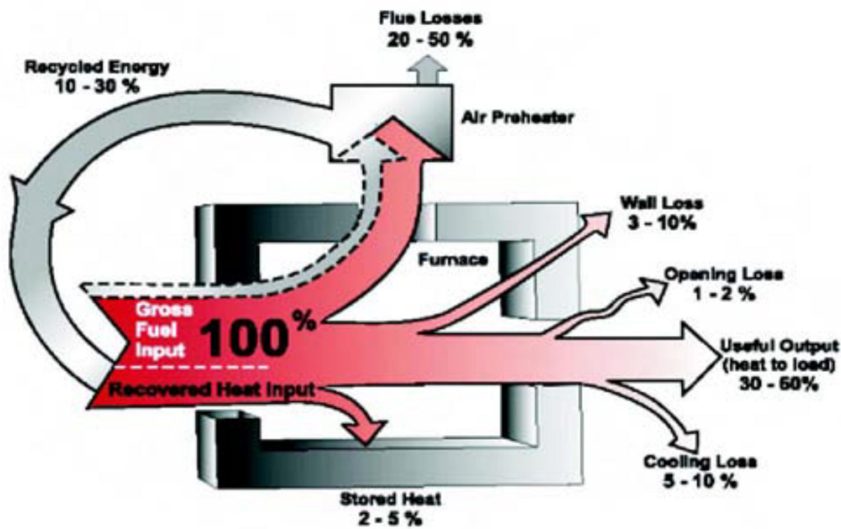
Figure 3.8: Fuel-fired furnace
