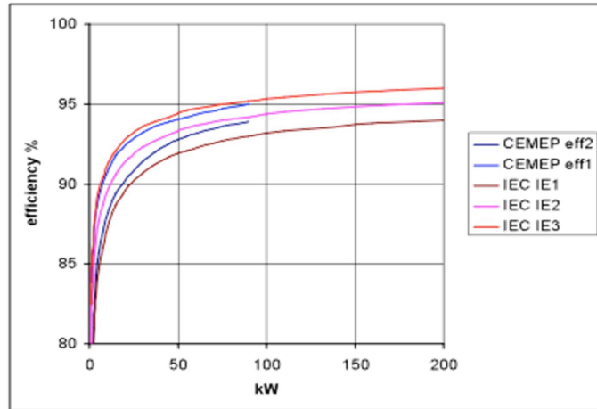
Figure 4.4: IEC motor efficiency classification
