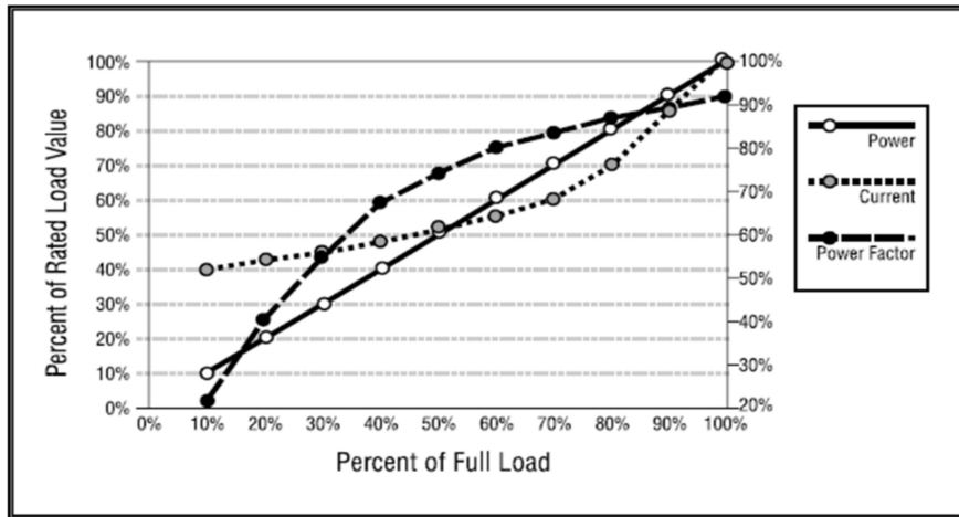
Figure 4.3: Typical induction motor characteristic curves
