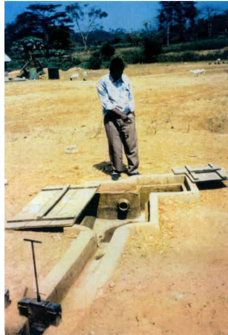
Fig. 3a: influent channel
