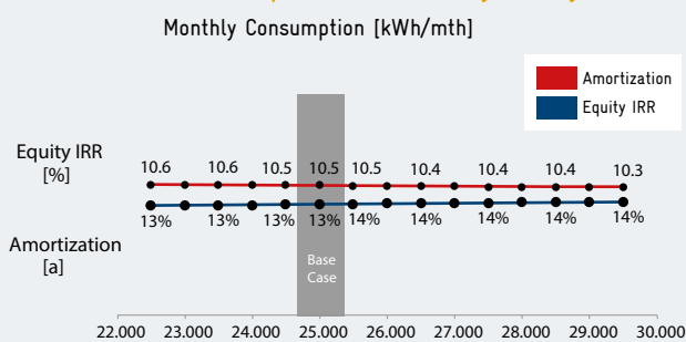
Figure 44: Mid-sized industrial PV system consumption sensitivity analysis
