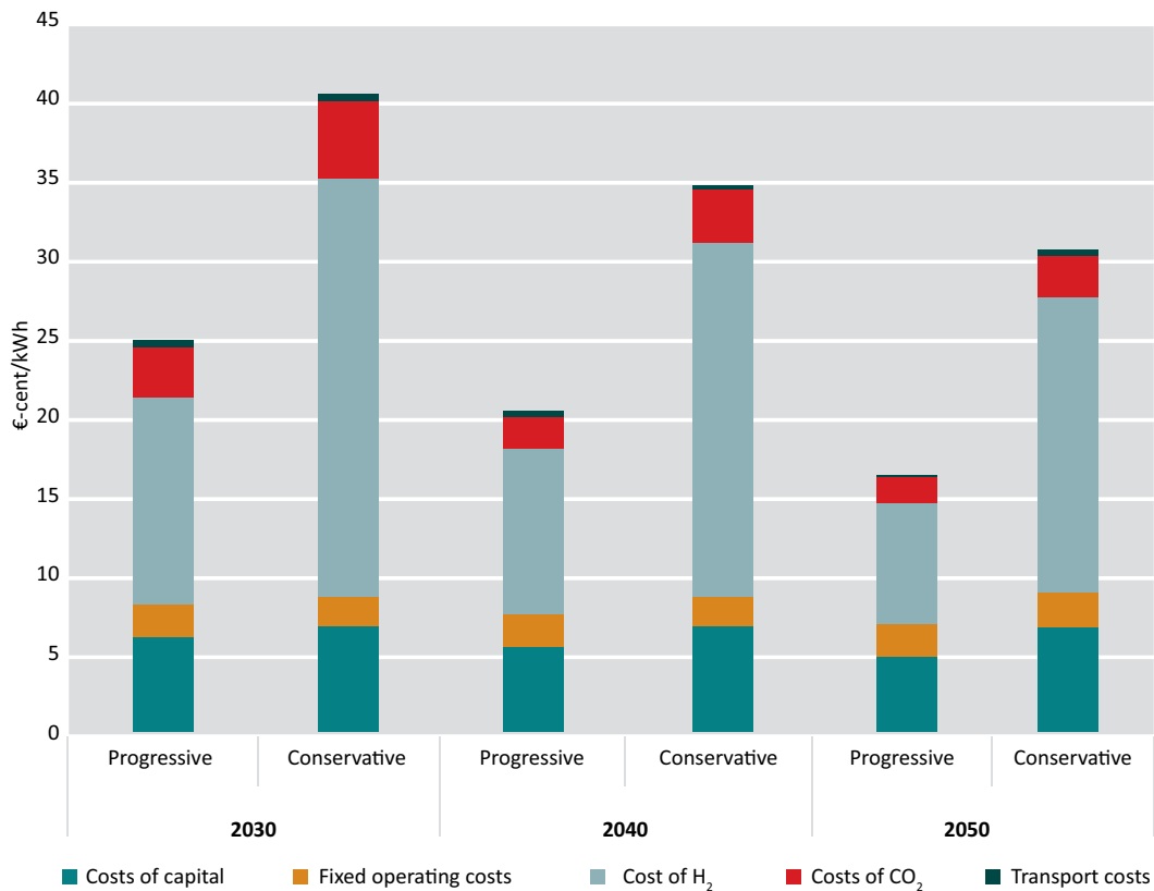
Fig. 6.11 Total costs of green synthetic kerosene
